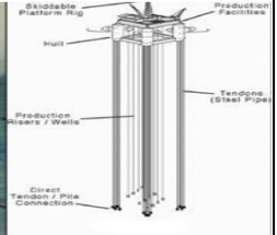
TLP
